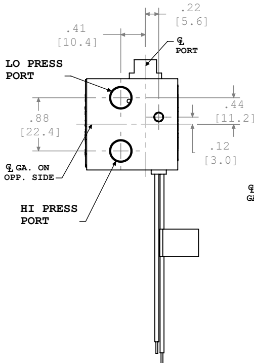
-4 PORTING (1/8" NPT)
