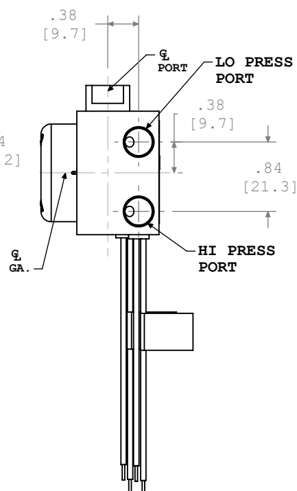
-5 PORTING (1/8" NPT)
