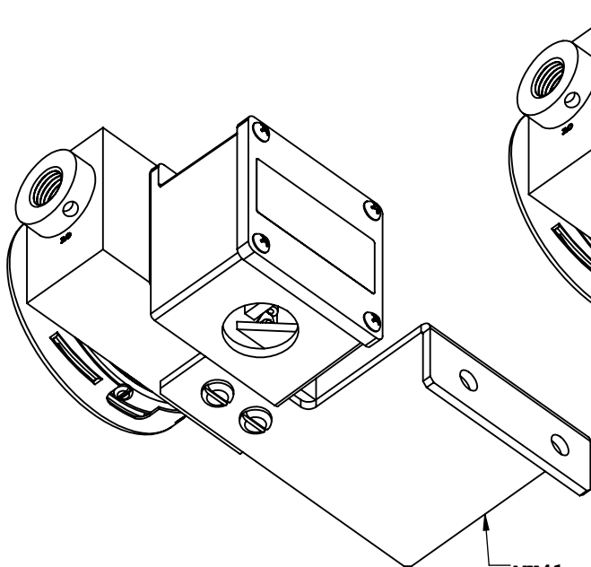
MK41 Flush Mount 1203/1303P(G)T Series
