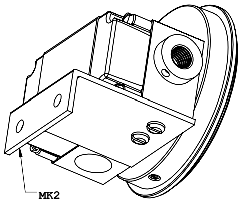
MK2 Flush Mount 1203/1303PG/PGS Series
